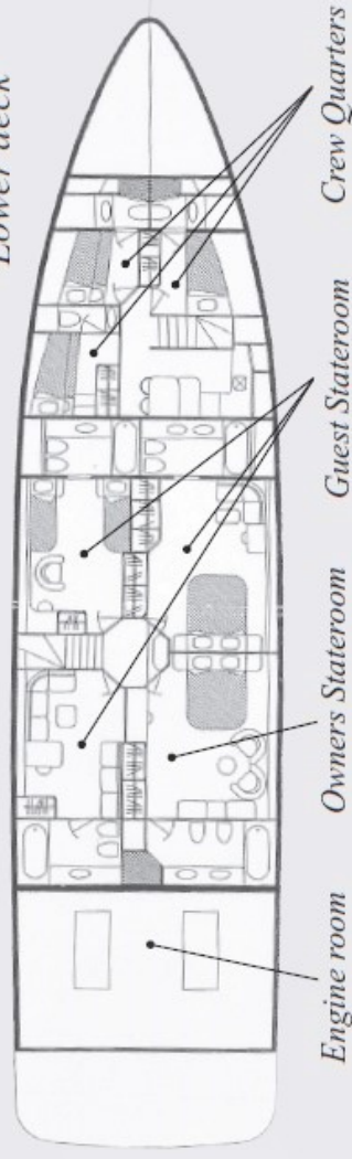
Lower deck
